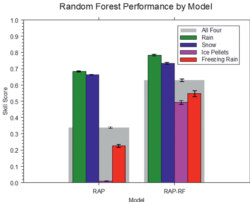
FIG. 6. Scores for the RAP postprocess ptype algorithm (left set of bars) and the RF ptype algorithm (right set of bars) based on mPING data for winter 2014/15. Score values are oriented such that larger positive numbers are better. The colored bars show the Pierce skill score for rain (green), snow (blue), ice pellets (magenta), and freezing rain (red). The gray bar is the Gerrity score for all four types taken together ordered as snow, rain, ice pellets, and freezing rain (Elmore et al. 2015).
