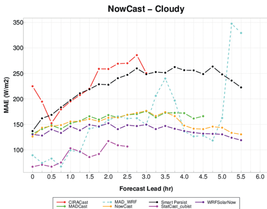
FIG. 7. Mean absolute error (MAE; \text{W m}^{-2} ) calculated over a 15-month period for all nowcast components aggregated over all sites (New York, Colorado, and California) for cloudy conditions. Note that StatCast performs the best, on average, for these difficult-to-forecast conditions.
