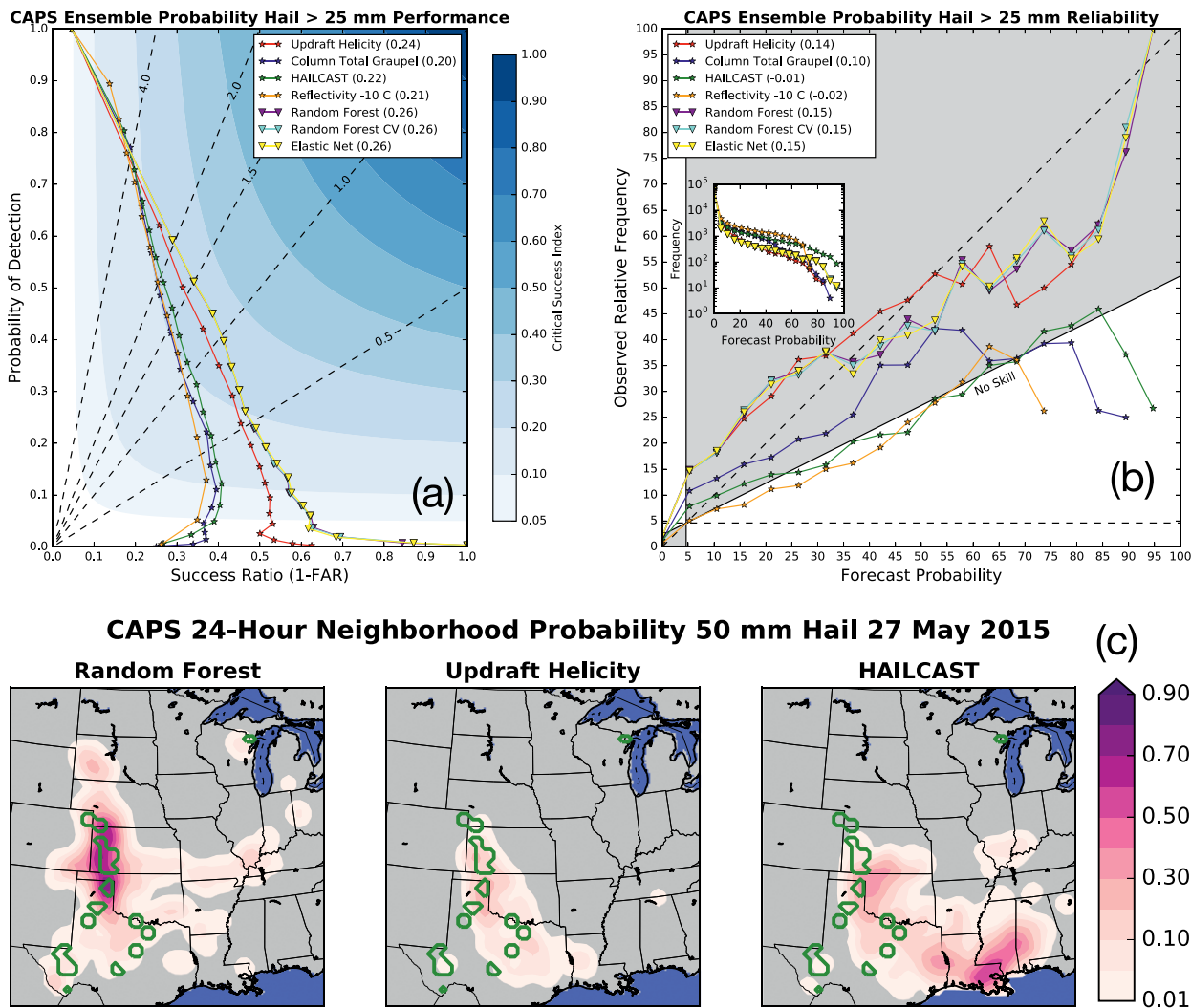
FIG. 5. (a) Performance diagram comparing different hail forecasting methods. (b) Attributes diagram indicating the reliability of different forecasting methods. (c) Forecast case showing the probability of 50-mm-or-larger hail in filled contours and observed 50-mm hail in green contours.
